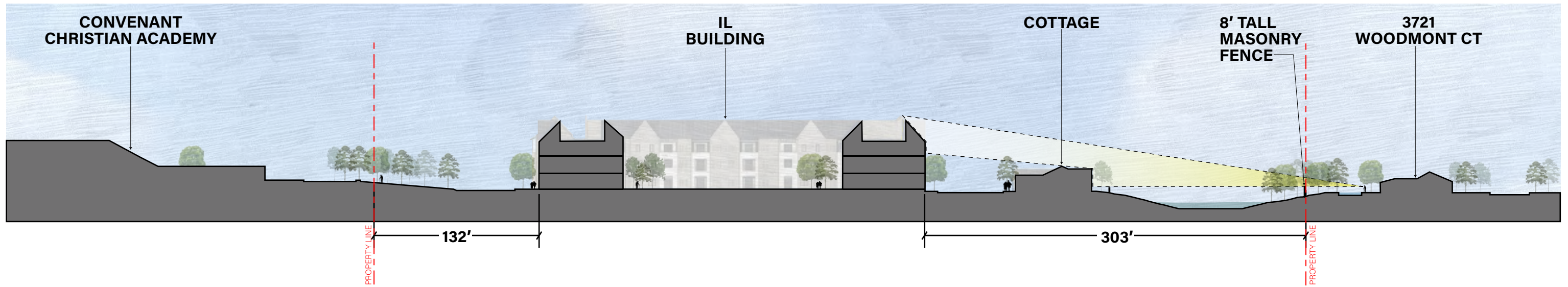
SECTION LOOKING NORTH
